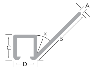
Reverse Angled Flange
