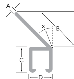
Angled Flange
